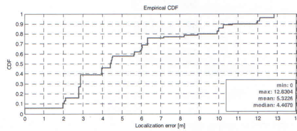
Fig. 10. CDF accuracy of GSM module
