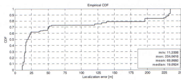
Fig. 11. CDF accuracy of Google module
