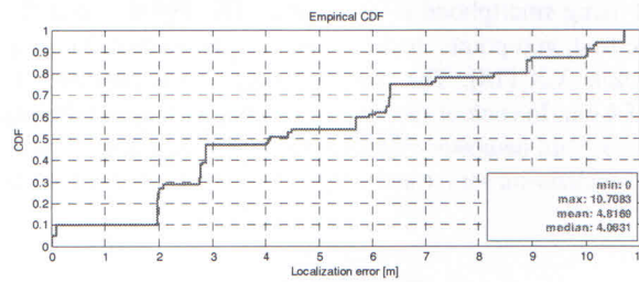
Fig. 9. CDF accuracy of Wi-Fi module
